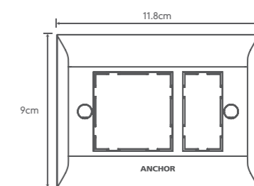
Single Mounting Plate Design
